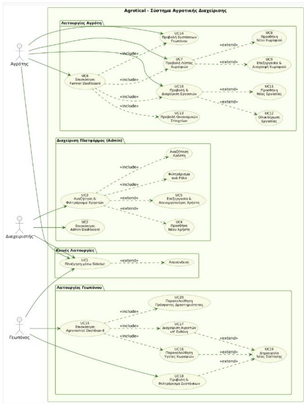
EIKONA1: USECASE DIAGRAM
